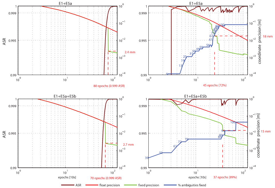
Figure 4. Galileo-only ambiguity success rates (ASR) and coordinate precision vs. number of epochs, for: E1 + E5a (top) and E1 + E5a + E5b (bottom), for a data sampling interval of 10 s. The left graphs relate to FAR, while the right graphs relate to PAR, both based on the criterion that ASR \geq 0.999 . See Figure 2 for an explanation of the different curves.
