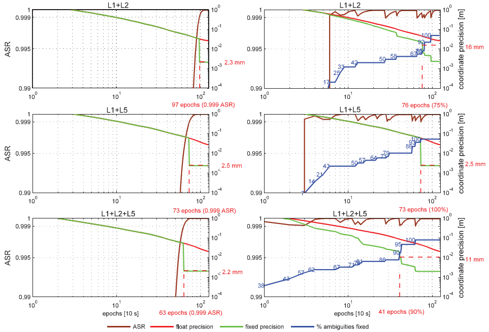
Figure 2. GPS-only ambiguity success rates (ASR) and coordinate precision vs. number of epochs, for: L1 + L2 (top), L1 + L5 (middle) and L1 + L2 + L5 (bottom), for a data sampling interval of 10 s. The left graphs relate to FAR, while the right graphs relate to PAR, both based on the criterion that ASR \geq 0.999 . The brown curve shows the ASR as a function of number of epochs within the batch, whilst the red curve depicts the float coordinate precision, and the green curve the (partially) fixed coordinate precision. Before this criterion is met, the fixed precision curve corresponds to its float counterpart. The blue curves on the right refer to the percentage of ambiguities that are (partially) fixed, i.e. \frac{n-p+1}{n} \times 100\% , with n the total number of ambiguities and where p equals the number of fixed ambiguities.
